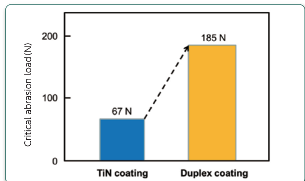
Fig.3 Effect of duplex treatment using atom nitriding
