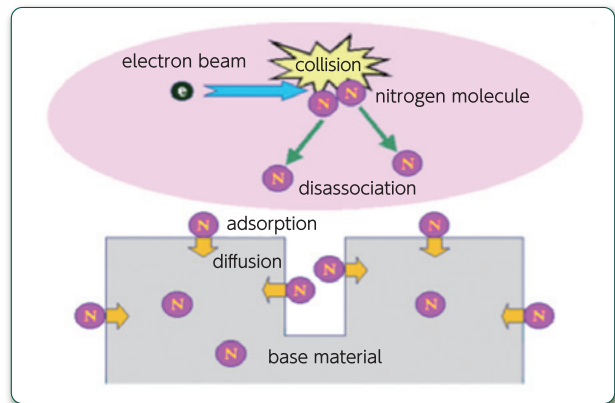
Fig.1 Principle of atom nitriding process
